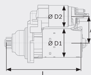
Noseless starter motor
