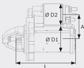
Nose-type starter motor
